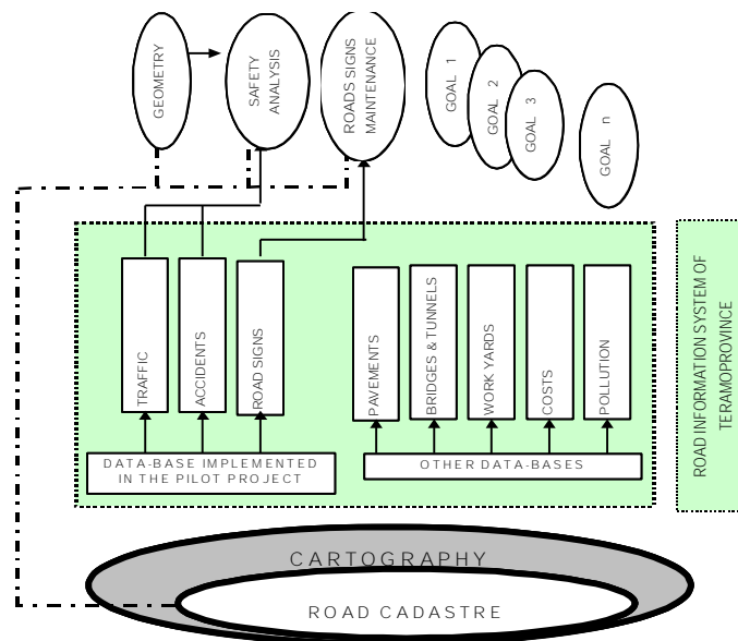
Fig. 2: Road Information System of Teramo Province
